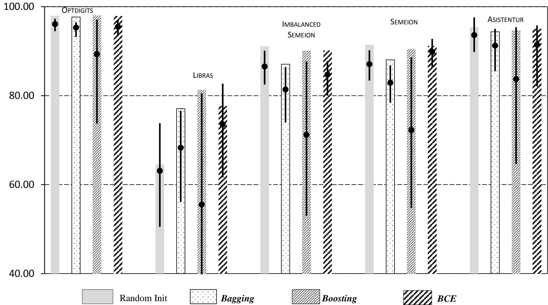
Fig 1.a. Ensemble Accuracy (bar), interval defined by the accuracy of the base learners (line) and the average accuracy of the base learners (point) when ensembles are built using the Full Feature Space
