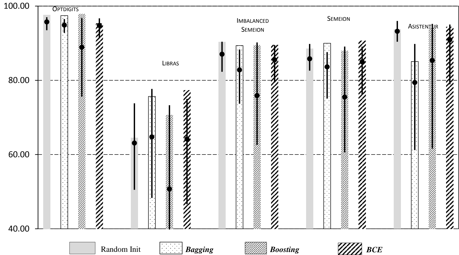
Fig. 1.b. Ensemble Accuracy (bar), interval defined by the accuracy of the base learners (line) and the average accuracy of the base learners (point) when ensembles are built using the Feature Subspace selected by CFS
